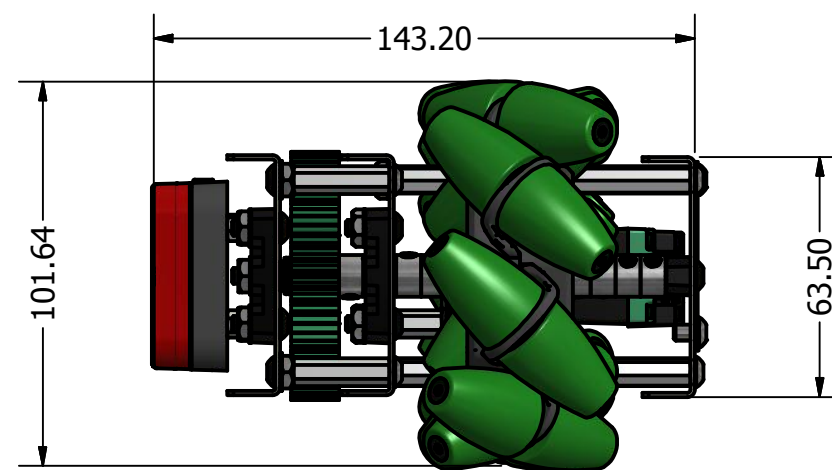
V. Frontal SCALE 1 / 2
