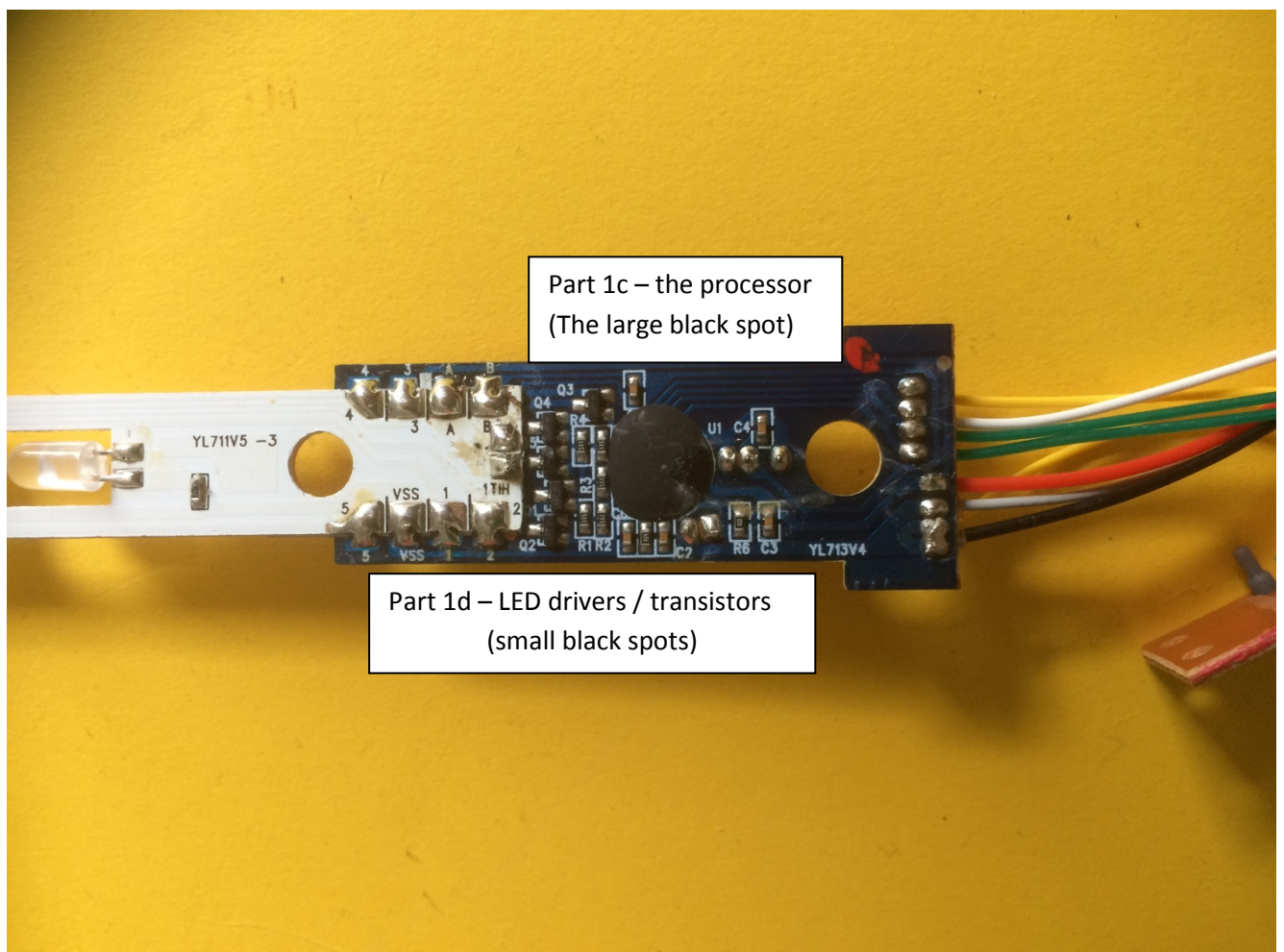
Photo 10 – front of circuit board
